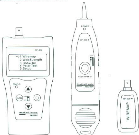
Main tester(NF-308)
